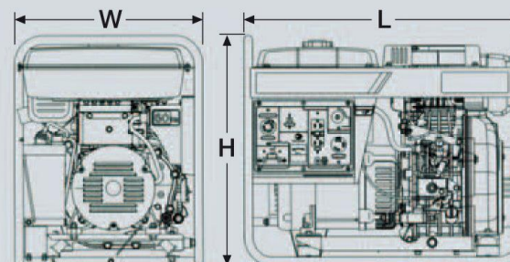
YDG-5500N / YDG-6600TN
